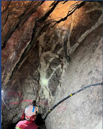
View of portion of Promontorio vein zone in immediate hanging wall of fault plane, Tirito shaft area.
