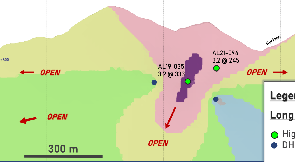
Coterá Target - AgEq* x Thickness Contours
