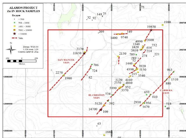
Figure 3. Zinc in rock samples, Yoreme concession.
