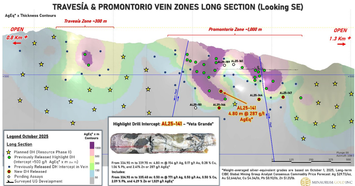
Figure 2. Longitudinal section of Travesia-Promontorio vein zones, showing locations of highlighted mineralized intersections.
