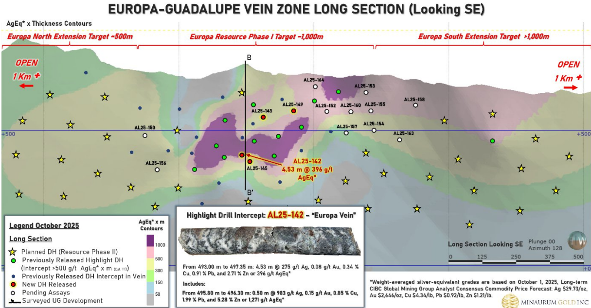
Figure 3. Longitudinal section of Europa vein zone, showing locations of highlighted mineralized intersections.
