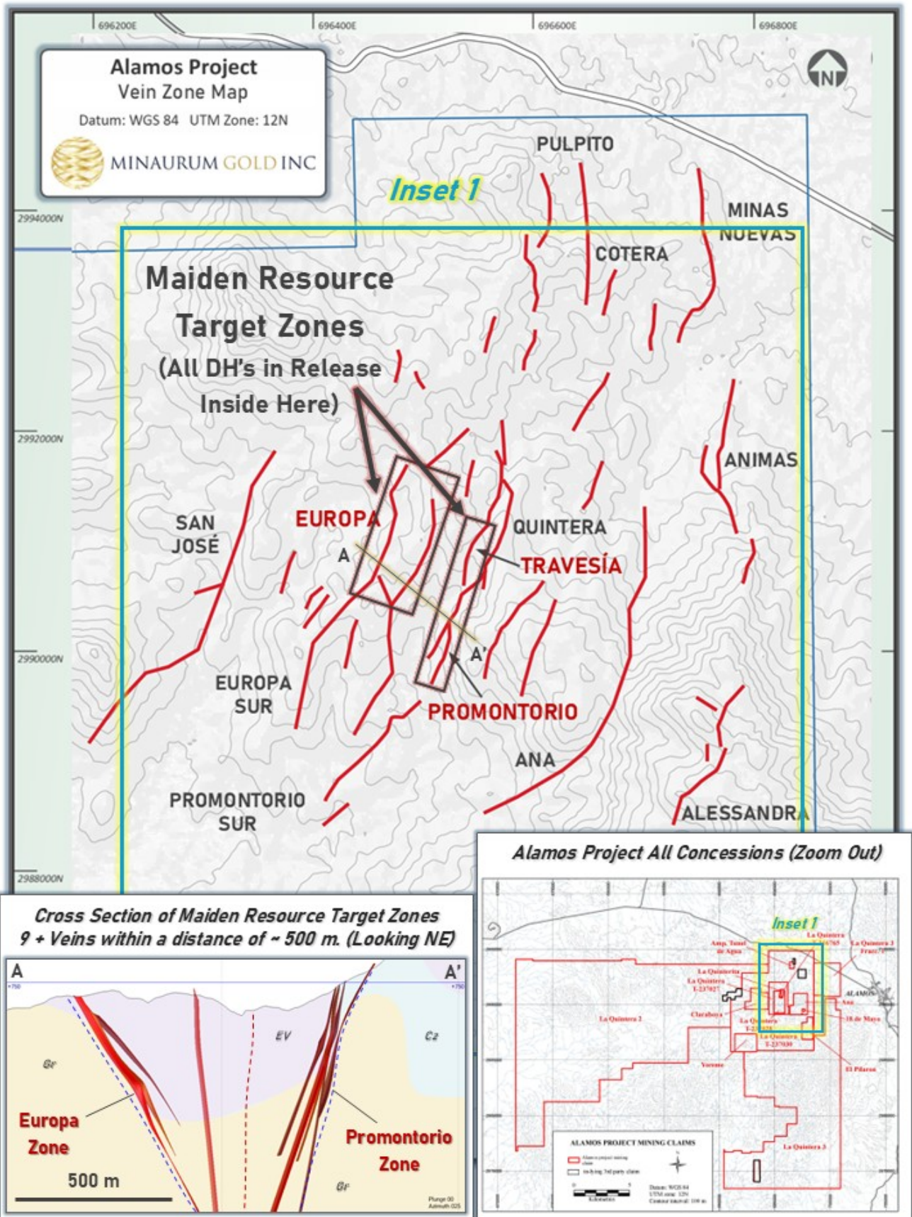
Figure 1. Plan view showing locations of Travesía, Promontorio, and Europa vein zones.
