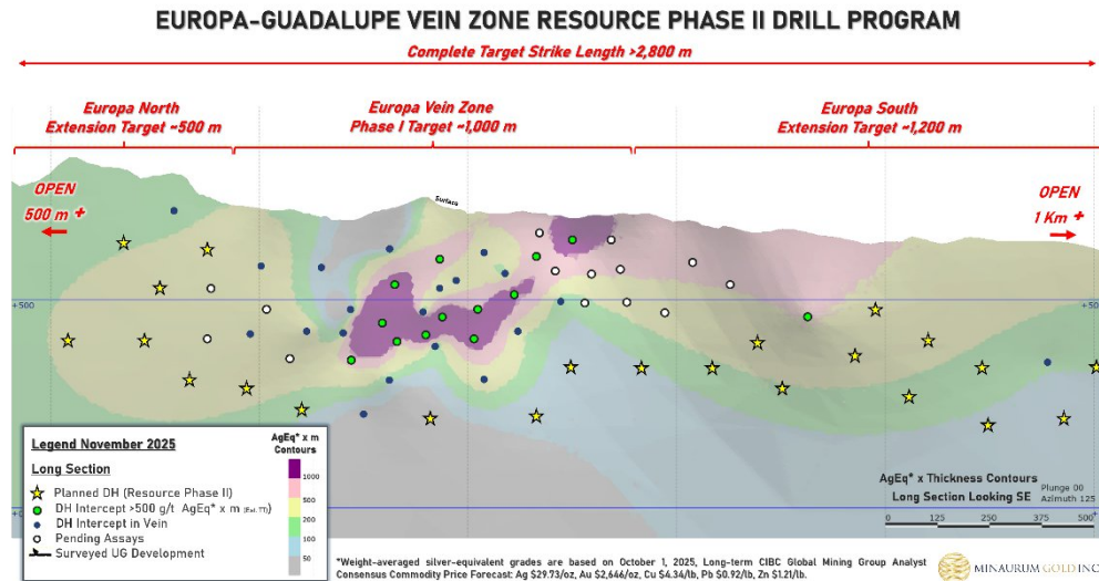
Figure 2. Europa vein zone longitudinal section.
