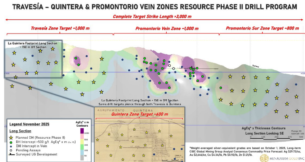
Figure 3. Travesía, Quintera and Promontorio vein zone longitudinal section.
